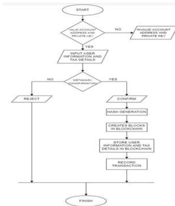
Figure 2: Flowchart
