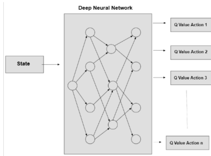
Figure 6: Deep Q learning (DQN)
