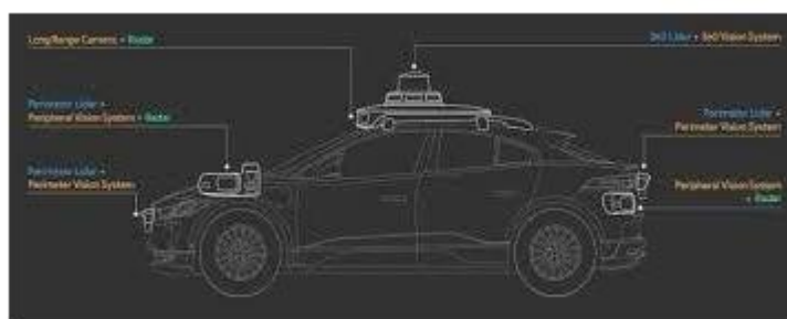
Figure 2: Diagram of the Sensor Suite in Waymo's Autonomous Vehicles, Highlighting the Various Technologies That Enable Real-Time Navigation and Decision-Making.
