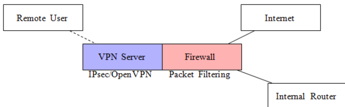
Figure 3: Network security architecture with firewall and VPN integration
