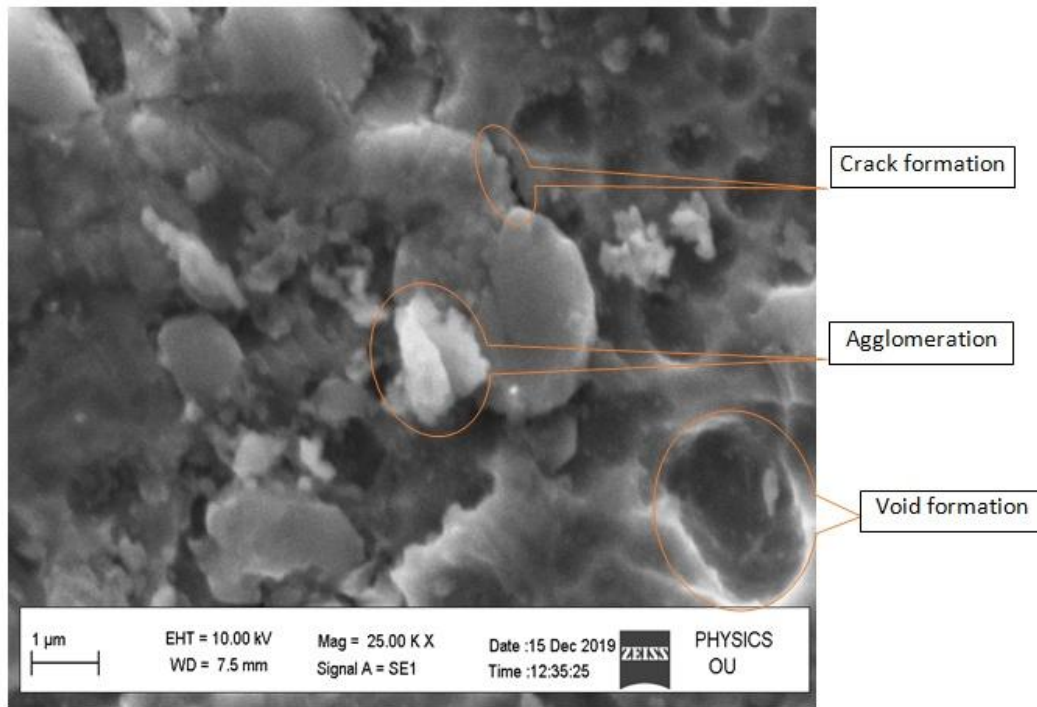
Figure 5.1: A 25000x SEM image of composite of LM 25 alloy with 1% Gr and 3% ZrO 2 . The various defects like crack formation, void formation and agglomeration of reinforcement material are visible in
