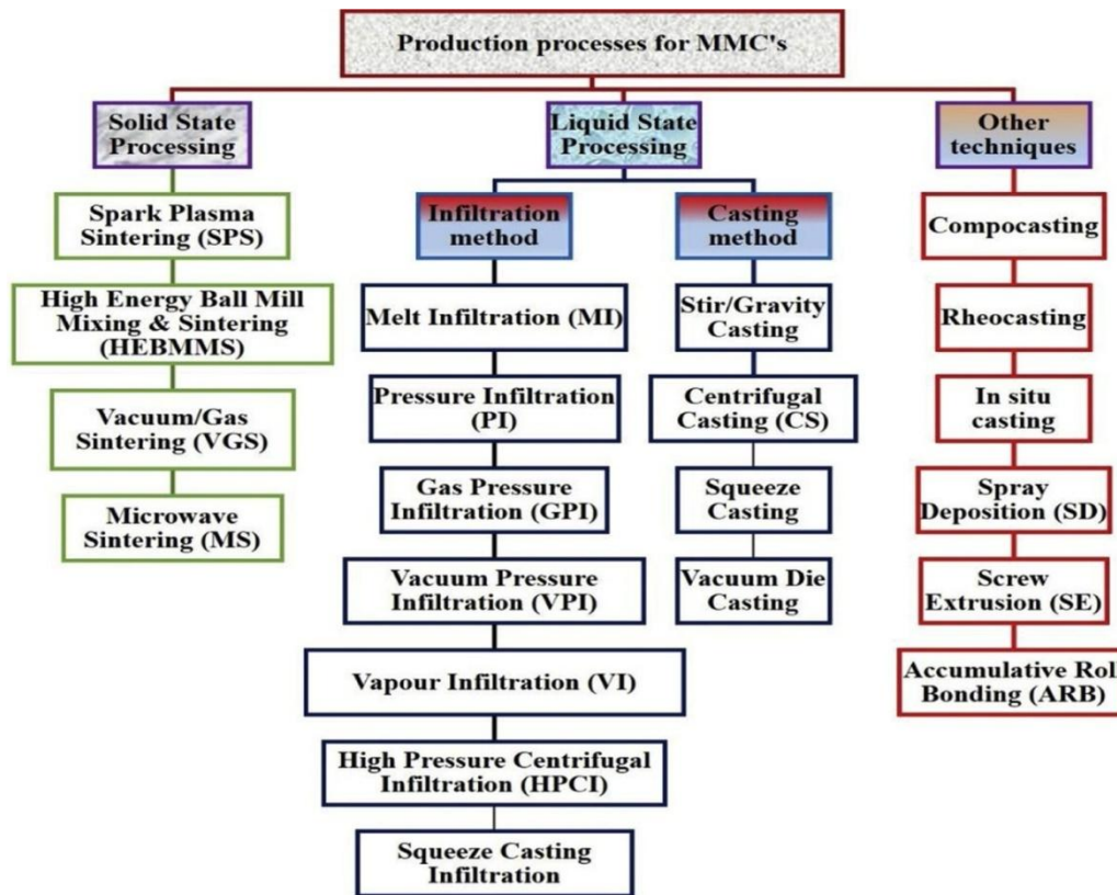
Figure 1.2: Classification of the various production process for MMCs
