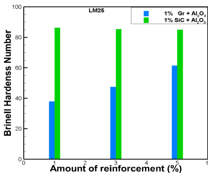
Figure 5.13: Variation of Brinell hardness number with amount of reinforcement of \text{Al}_2\text{O}_3 in LM25 + 1% Gr and 1% SiC alloy
