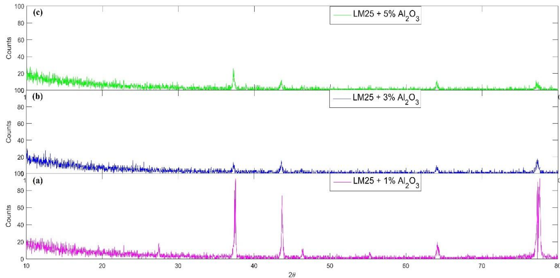
Figure 5.5: XRD data for composite of LM 25 alloy using \text{Al}_2\text{O}_3 with (a) 1% (b) 3% (c) 5% \text{Al}_2\text{O}_3 . The
