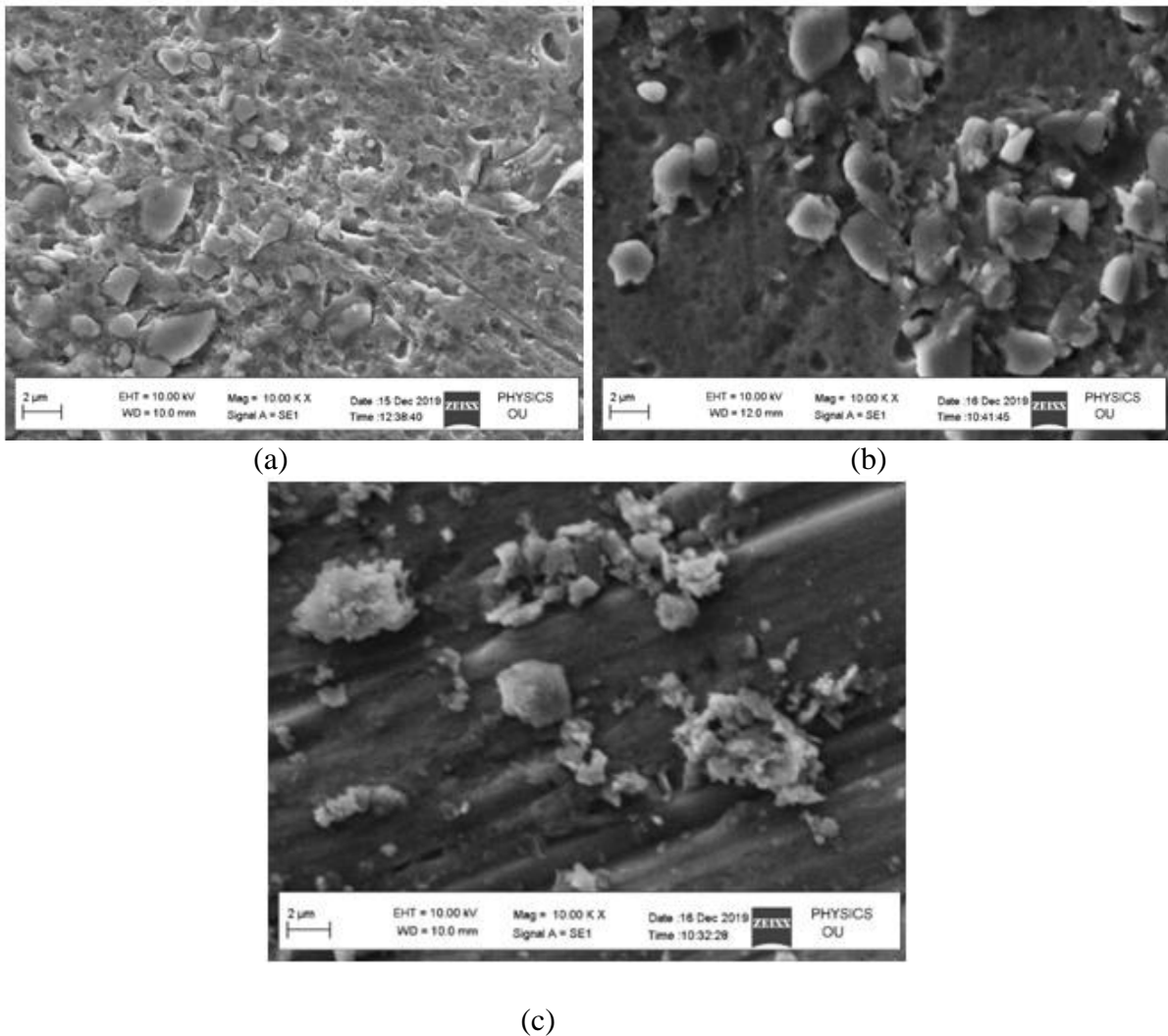
Figure 5.3: A SEM image of composites of LM 25 alloy with (a) 1% Gr and 5% \text{ZrO}_2 (b) 1% SiC and 5% \text{Al}_2\text{O}_3 (c) 5% \text{Al}_2\text{O}_3
