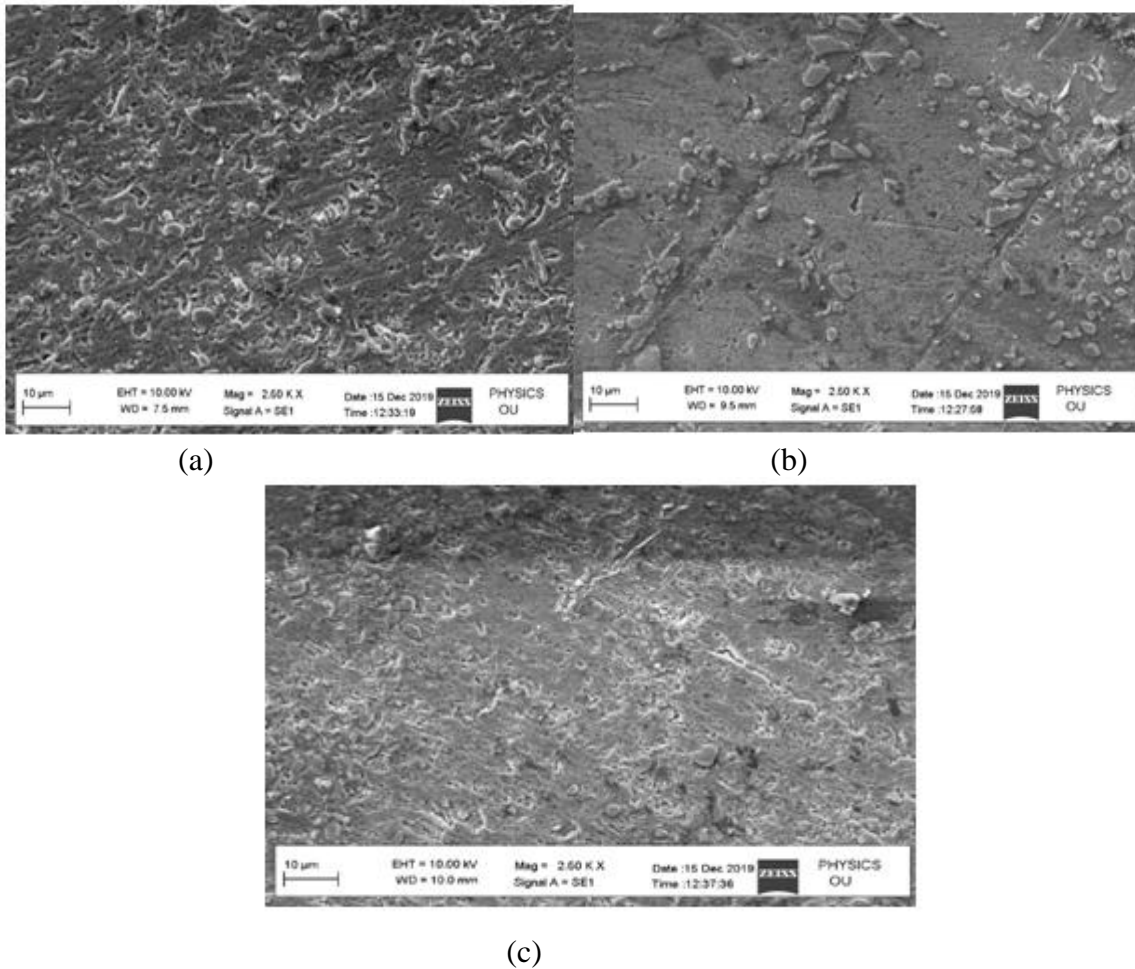
Figure 5.2: 2500x SEM image of composites of LM 25 alloy with 1% Gr and ZrO_2 of (a) 1% (b) 3% (c) 5%
