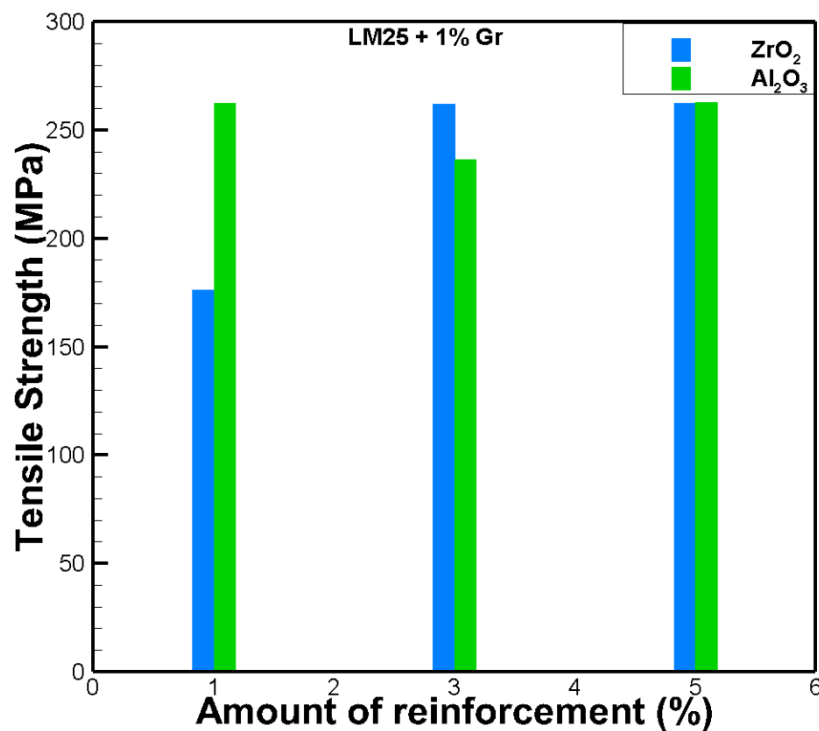
Figure 5.8: Variation of tensile strength with amount of reinforcement of \text{ZrO}_2 and \text{Al}_2\text{O}_3 in LM25 + 1% Gr alloy
