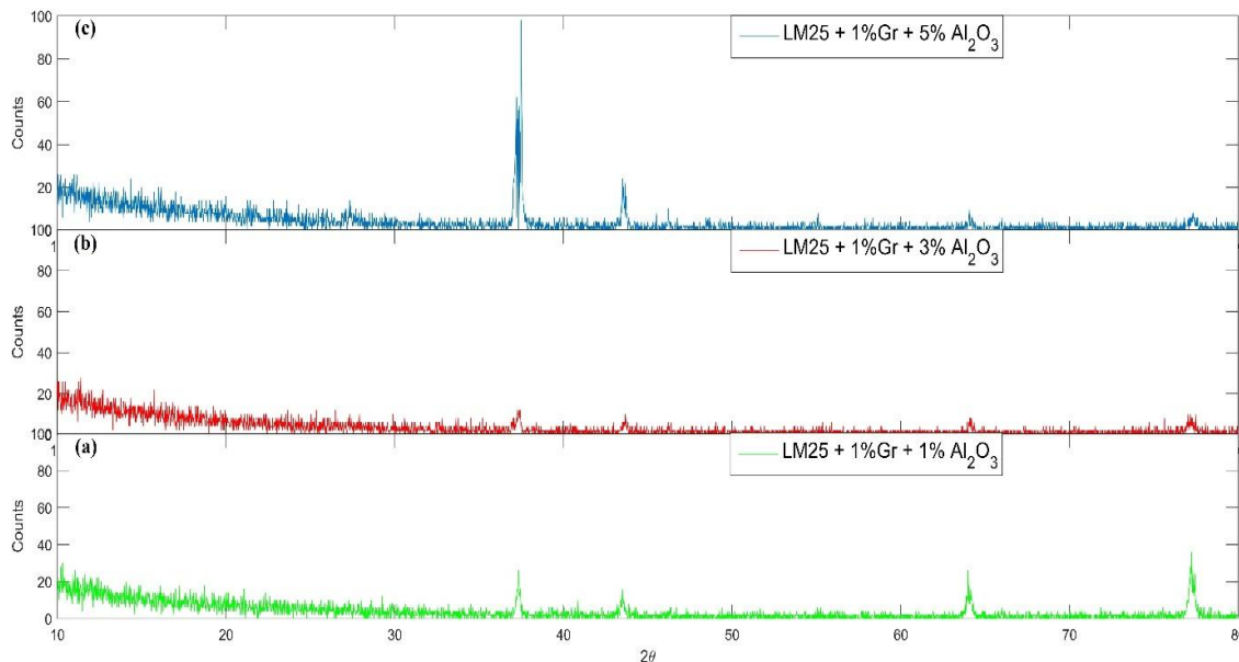
Figure 5.6: XRD data for composite of LM 25 alloy using 1% Gr and \text{Al}_2\text{O}_3 with (a) 1% (b) 3% (c) 5% \text{Al}_2\text{O}_3 .
