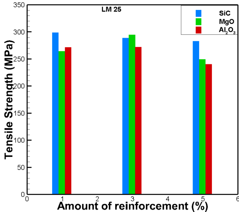
Figure 5.7: Variation of tensile strength with amount of reinforcement of SiC, MgO and \text{Al}_2\text{O}_3 in LM25 alloy
