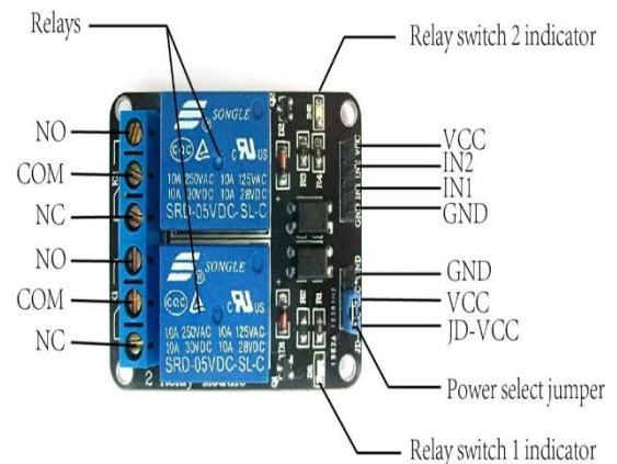
Figure 3: 2-channel relay
