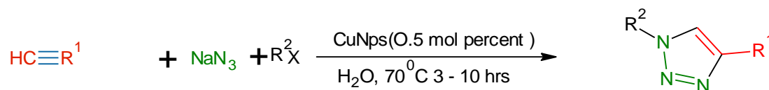
Scheme 14 : Synthesis of substituted triazoles using Cu NPs
