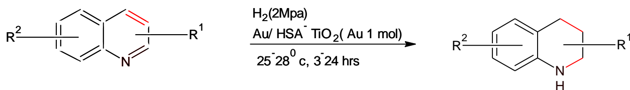
Scheme 6: 3 Hydrogenation of quinolines (35a) catalyzed by Au NPs
