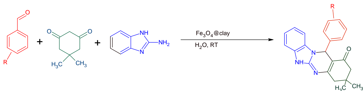
Scheme 36: Synthesis of imidazo(thiazolo)pyrimidines by using \text{Fe}_3\text{O}_4@ clay nanocatalyst
