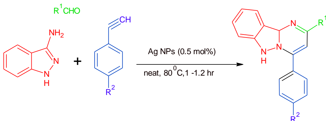
Scheme 1: Synthesis of pyrimido[1,2-b] indazole by using Ag NPs under solvent free condition
