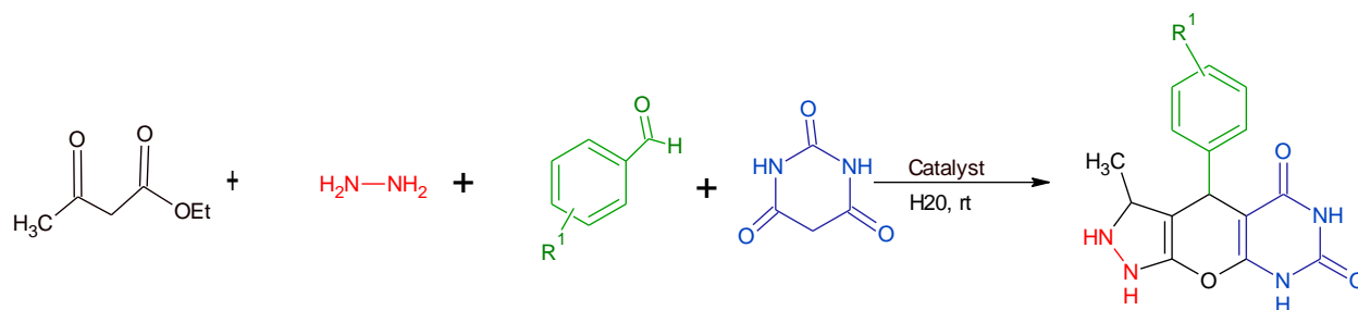
Scheme13: Synthesis of pyrazolopyranopyrimidine-5,7-diones.
