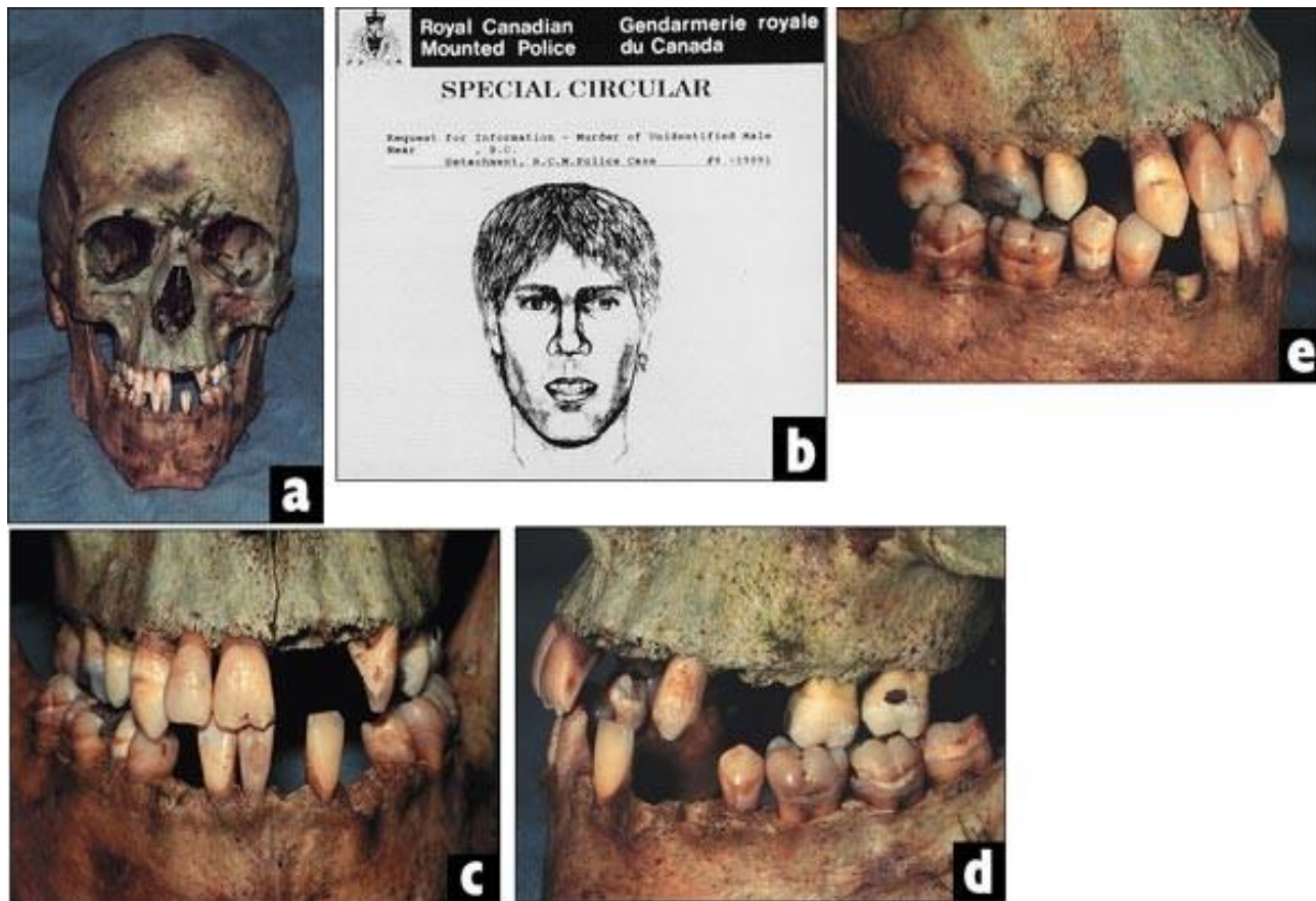
Figure 3: Dental Profiling
