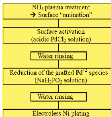
Figure 1. Technical process of electroless Ni-P coatings
